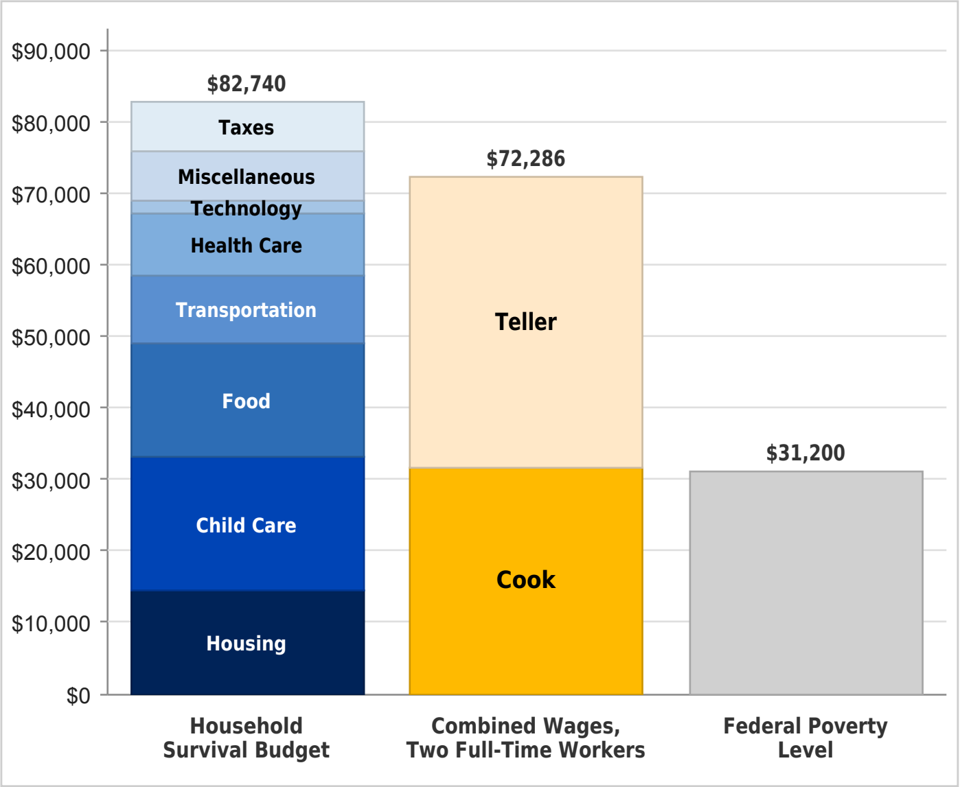
Figure 2. Household Survival Budget Costs Exceeded Wages of Common Jobs and the FPL Family of Four, Pennsylvania, 2024
